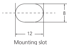
Mounting slot
